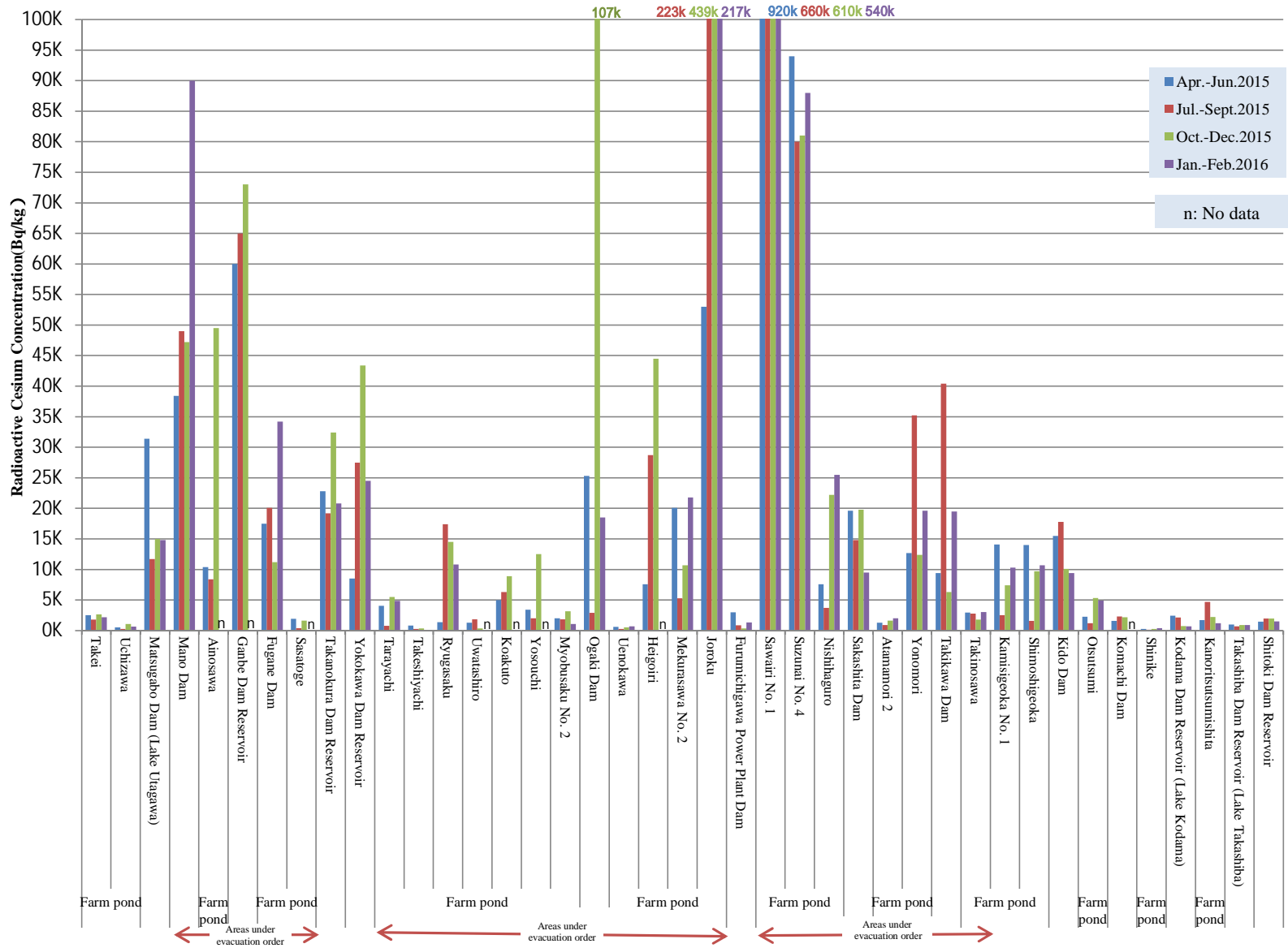
Lakes(Sediment):Changes in radioactive cesium concentration (Hamadori,Fukushima Prefecture)(FY2015)
