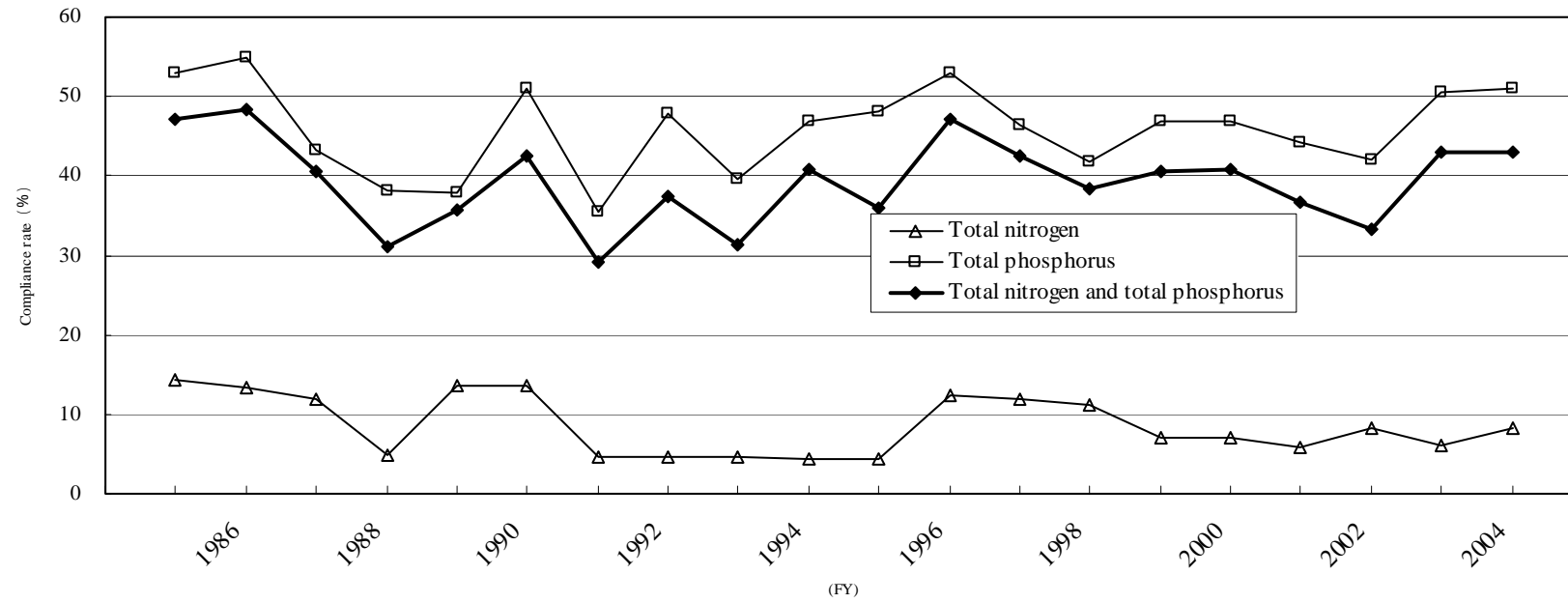
Fig. 3 Changes in Environmental Quality Standards Compliance Rate of Total Nitrogen and Total Phosphorus in Lakes and Reservoirs
