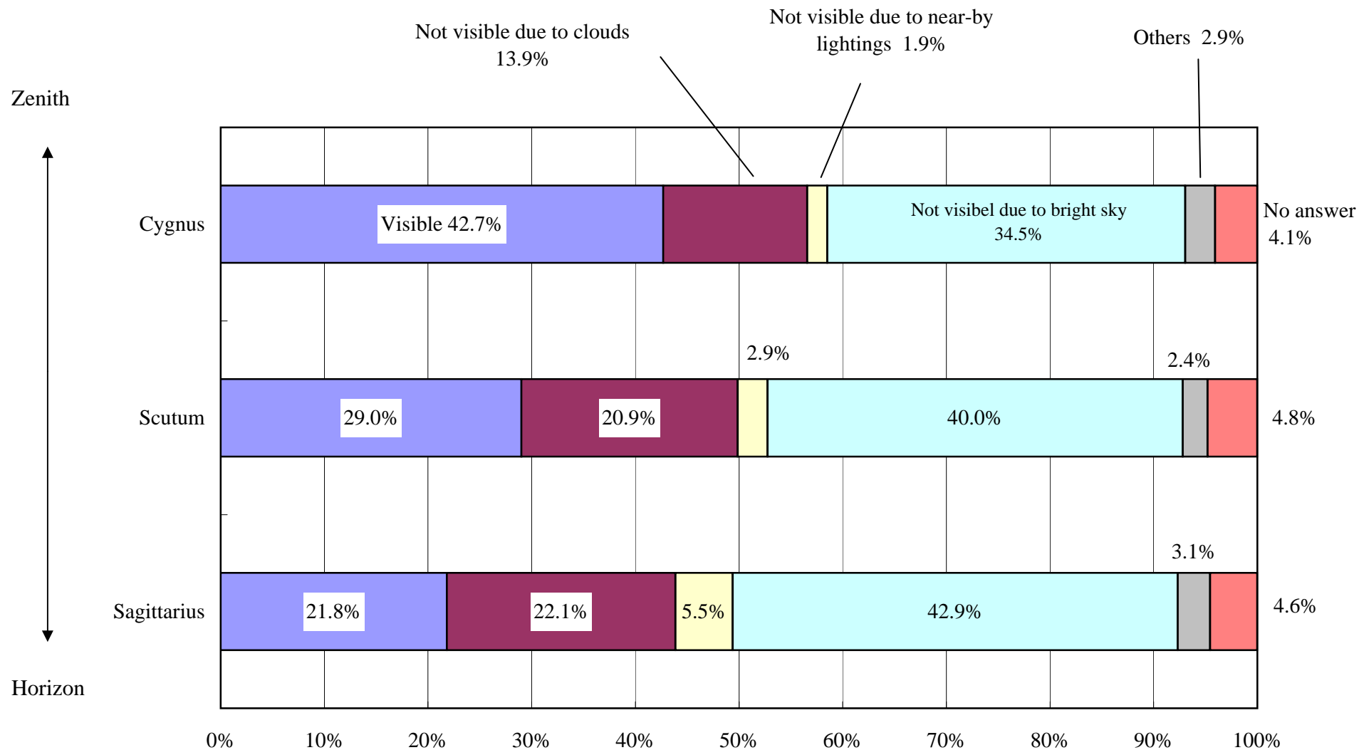
Fig. 1 Naked Eye Observation of the Milky Way
