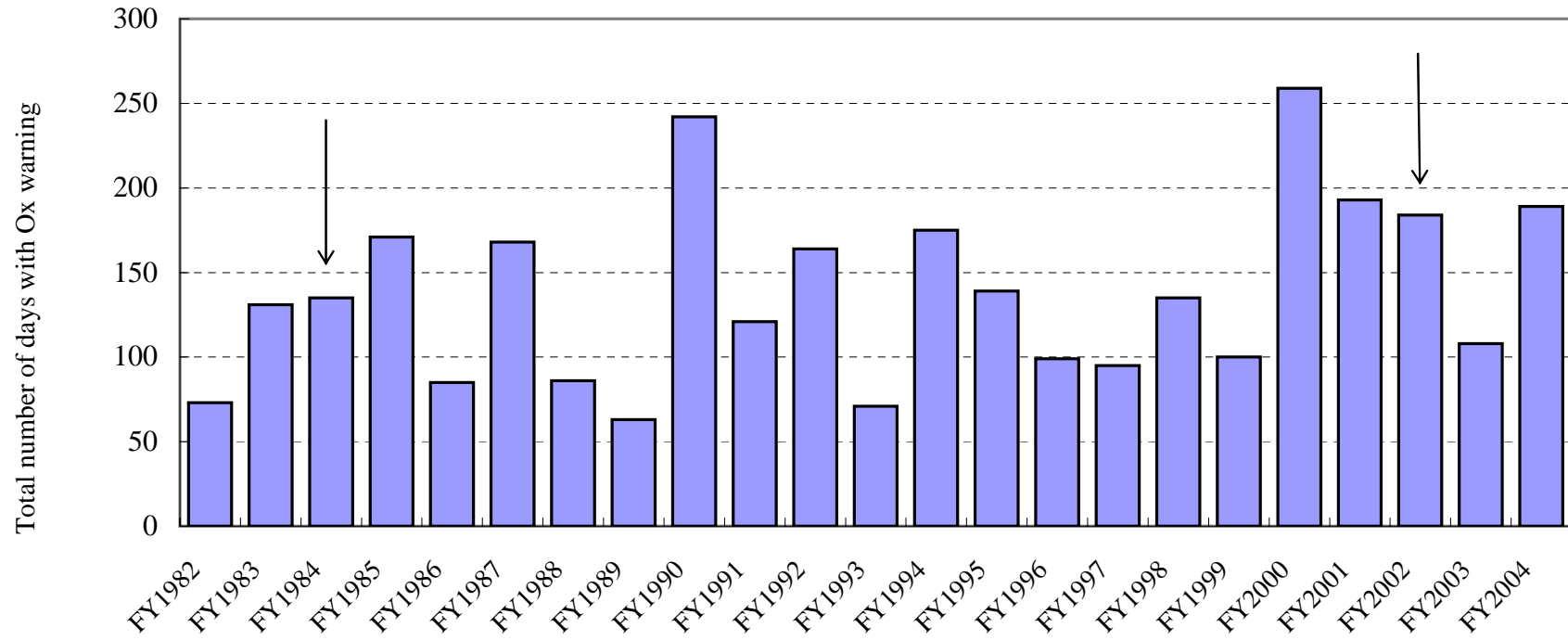
Fig. 3-2 Changes in Number of Days Photochemical Oxidant (Ox) Warning Issued
