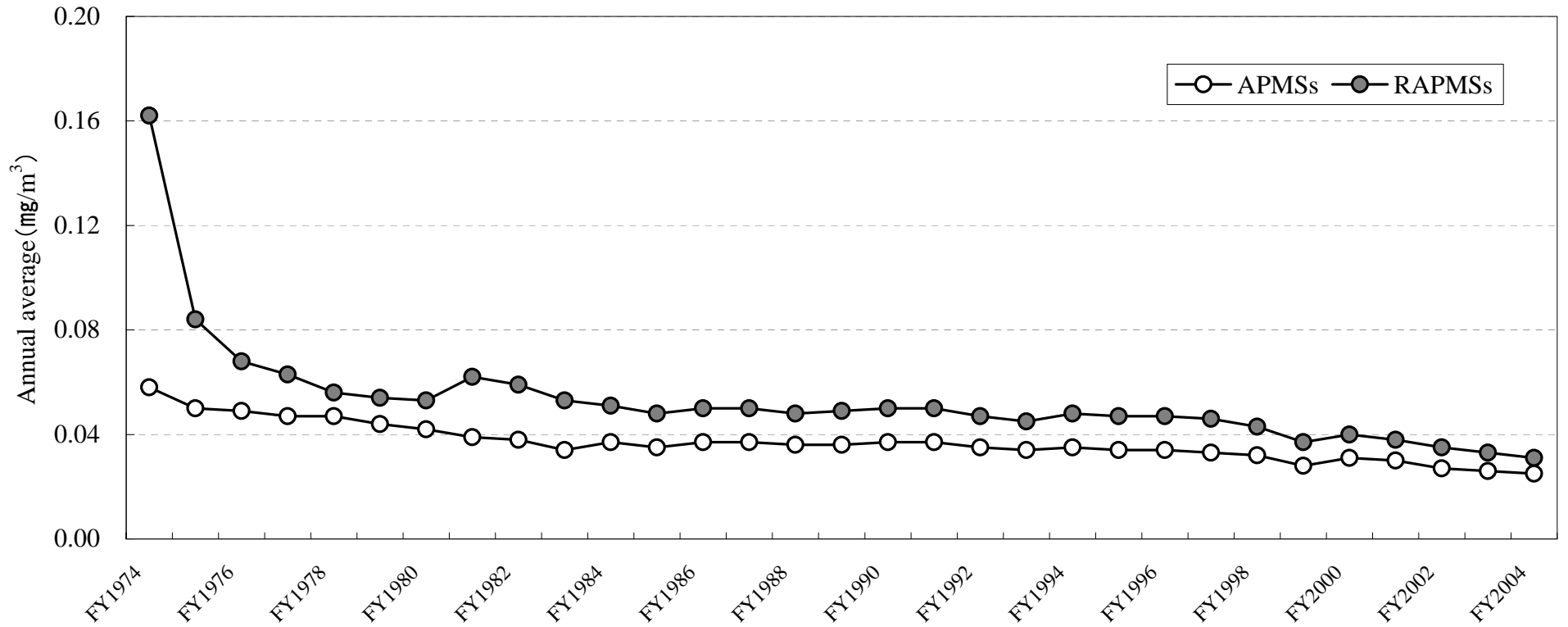
Fig. 2-2 Change in Annual Average Concentration of Suspended Particulate Matter
