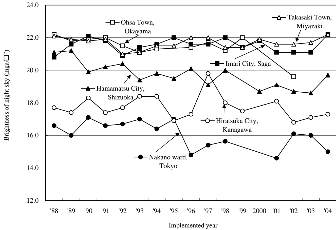
Fig. 3 Changes of Brightness of Night Sky Observed at Fixed Observation Point
