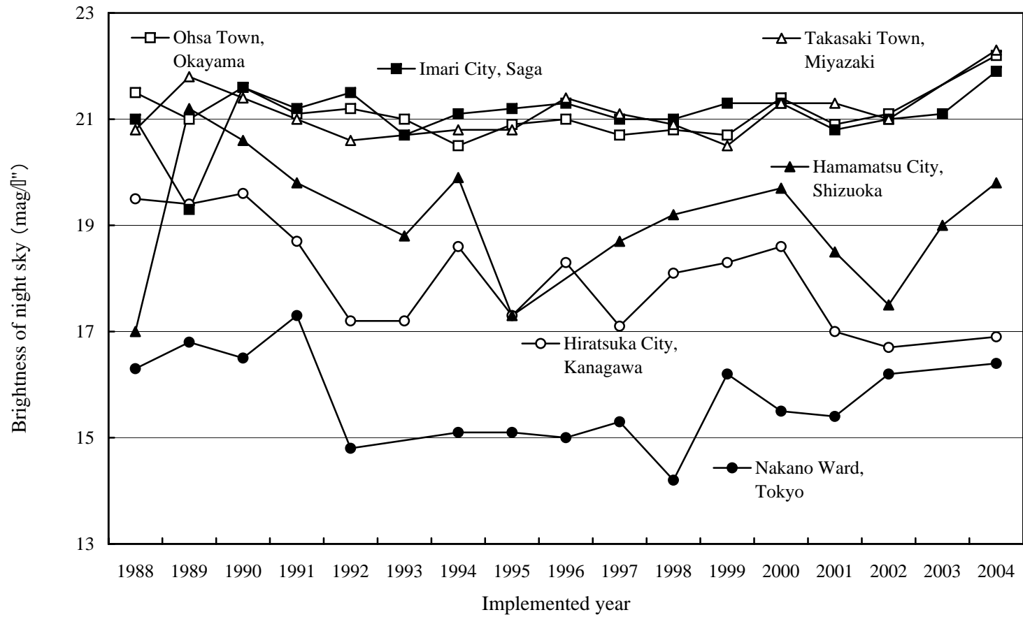
Fig.3 Changes of Brightness of Night Sky in Fixed Observation Point (Summer)
