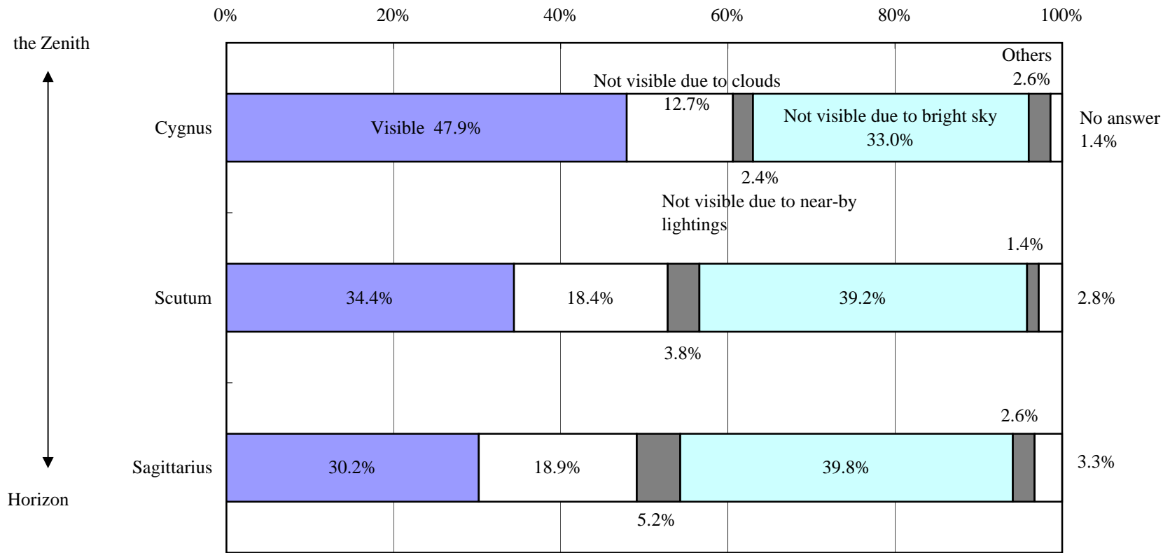
Fig.1 Naked Eye Observation of the Milky Way
