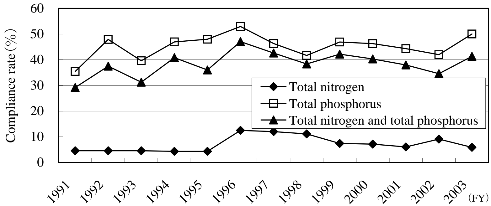
Fig. 3 Changes in Environmental Quality Standards (EQSs) Compliance Rates of Total Nitrogen and Total Phosphorus in Lakes and Reservoirs
