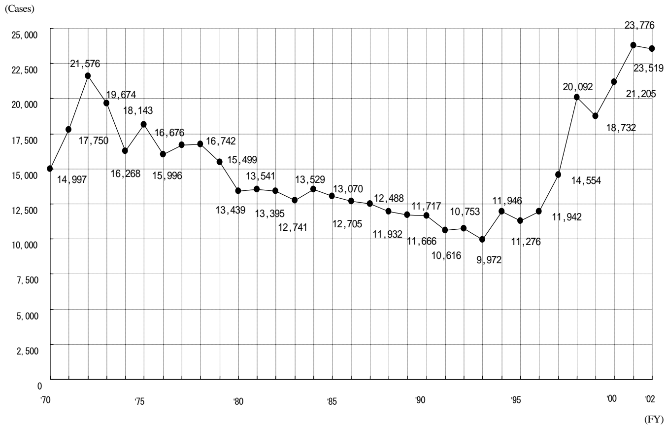
Fig. 1 Trend in Number of Complaints on Offensive Odor
