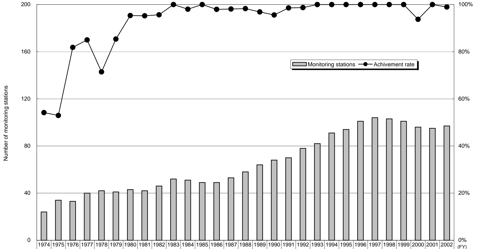
Fig.4-3 Achievement Rate of the Environmental Quality Standard for Sulfur Dioxide (SO 2 ) (roadside air pollution monitoring stations)
