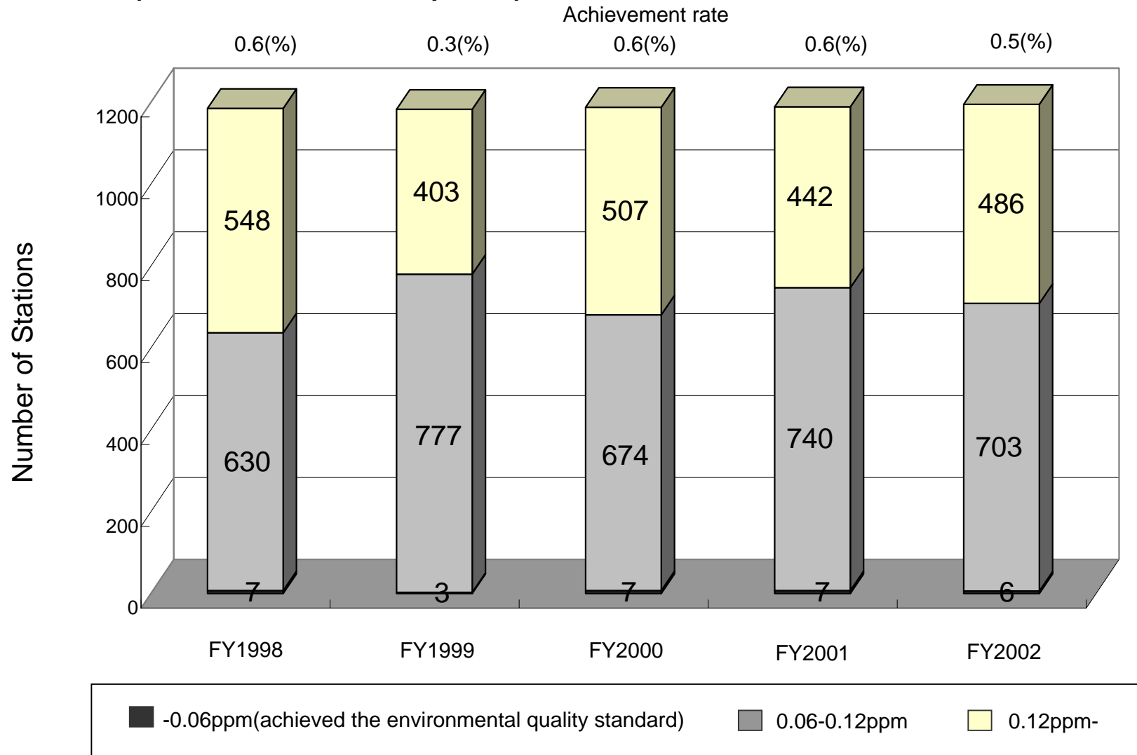
Fig.3 Number of Monitoring Stations (APMSs+RAPMSs) by Photochemical Oxidant Levels (Maximum value of hourly value)
