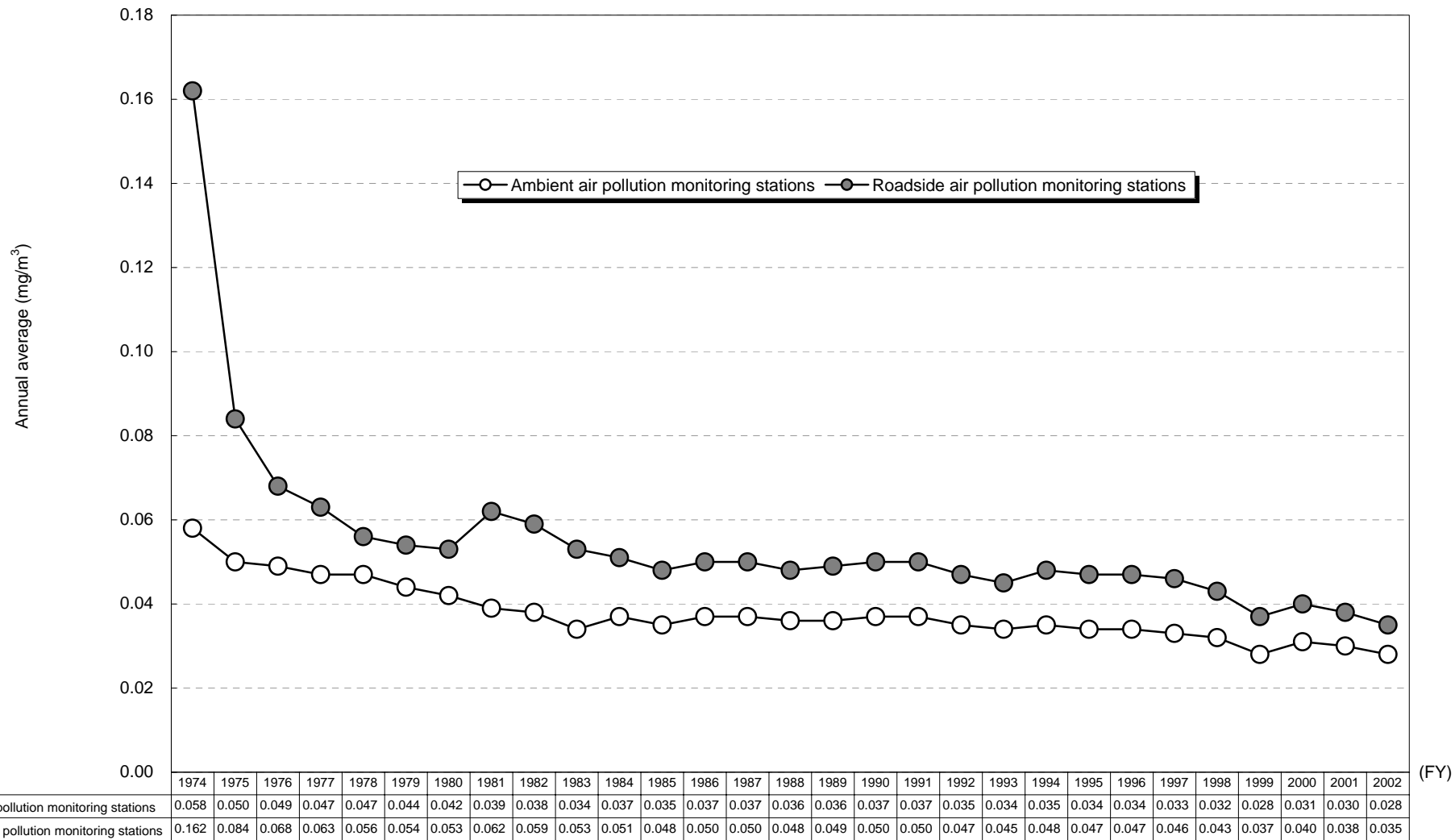
Fig. 2-1 Change in Annual Average of Suspended Particulate Matter (SPM) Concentration
