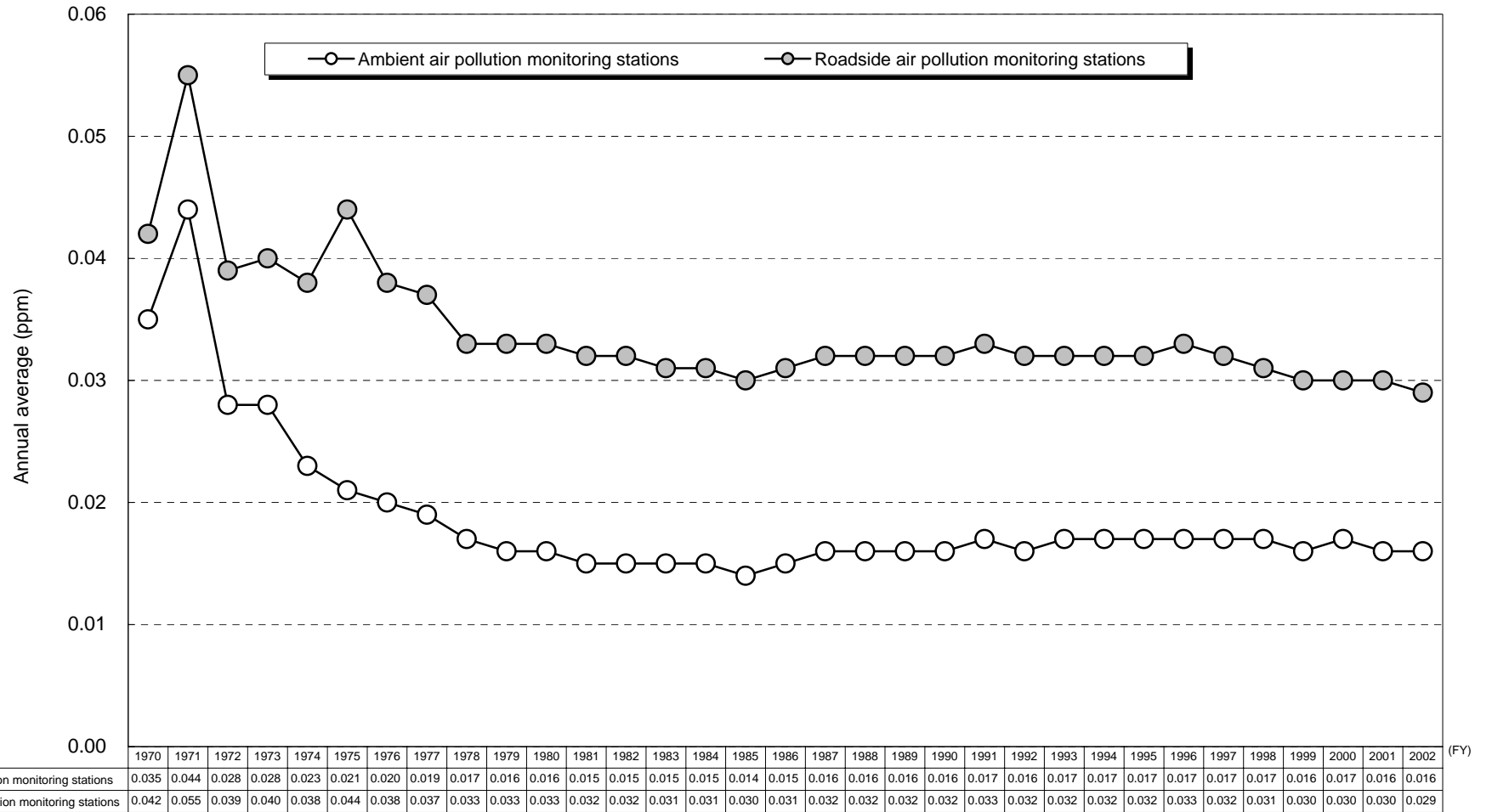
Fig.1-1 Change in Annual Average of Nitrogen Dioxide (NO 2 ) Concentration
