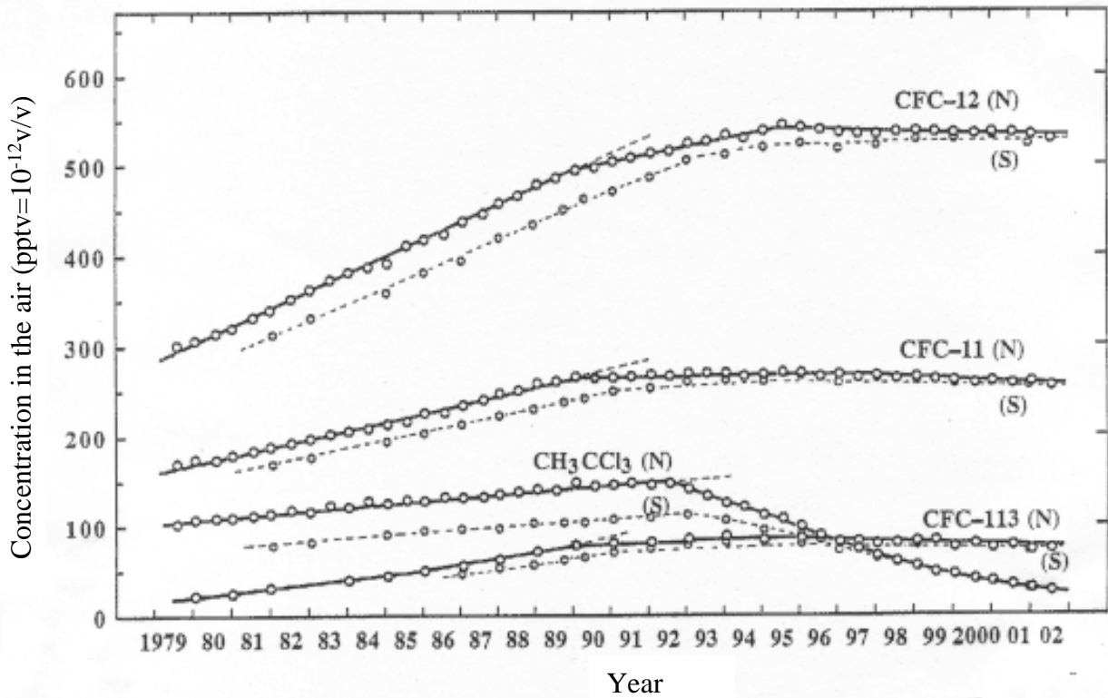
Fig. 3 Secular Change of the Average Concentrations of Specified Substances in the Atmosphere at Mid-latitudes in the Northern Hemisphere (N=Hokkaido) and in the Southern Hemisphere (S=Showa Base in Antarctica)
