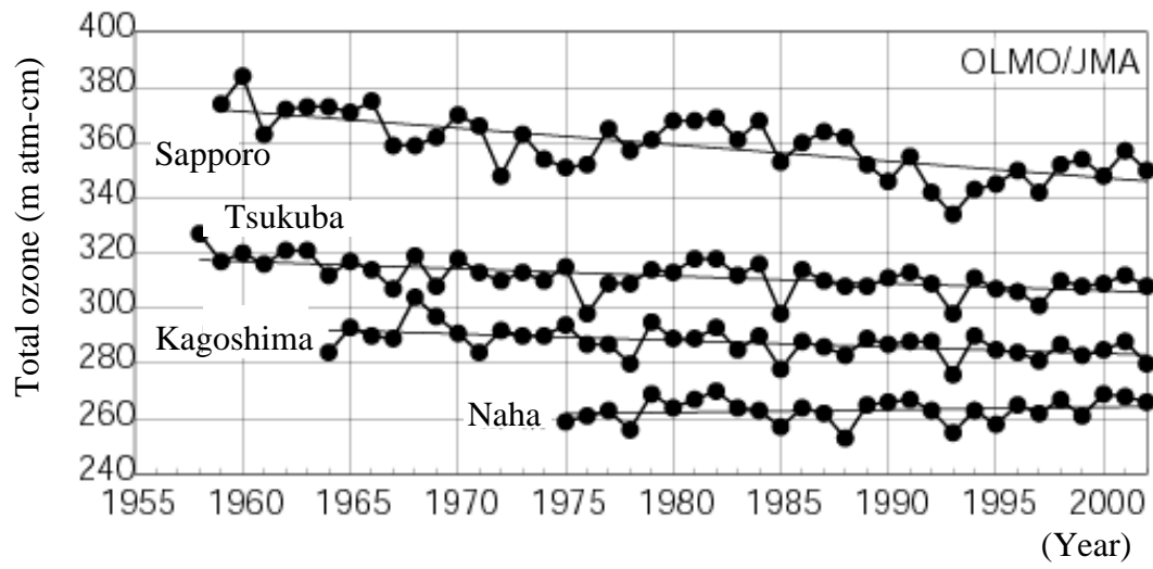
Fig. 2 Change in Annual Averages of Total Ozone over Japan (1958-2002)
