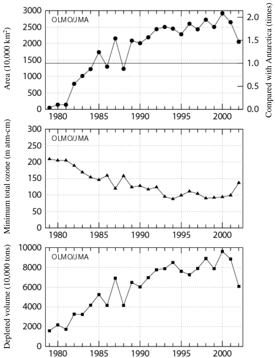
Fig.1 Secular Change of the Three Elements of Ozone Hole Depletion over Antarctica (1979-2002)
