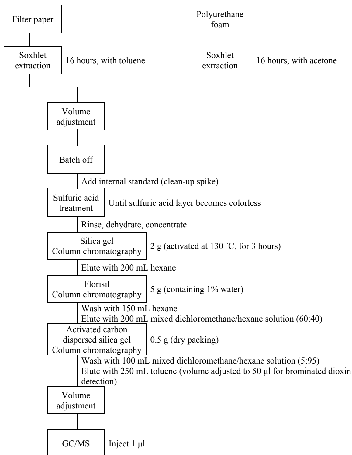
Figure 9. Flowchart of analytical method for determining brominated dioxins in ambient air and settled soot and dust
