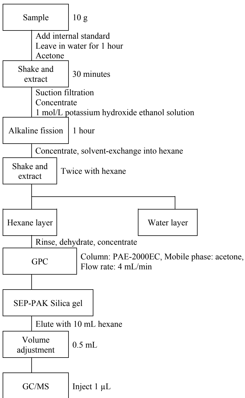
Figure 18. Flowchart of analytical method for determining polybrominated diphenyl ethers in sediment samples
