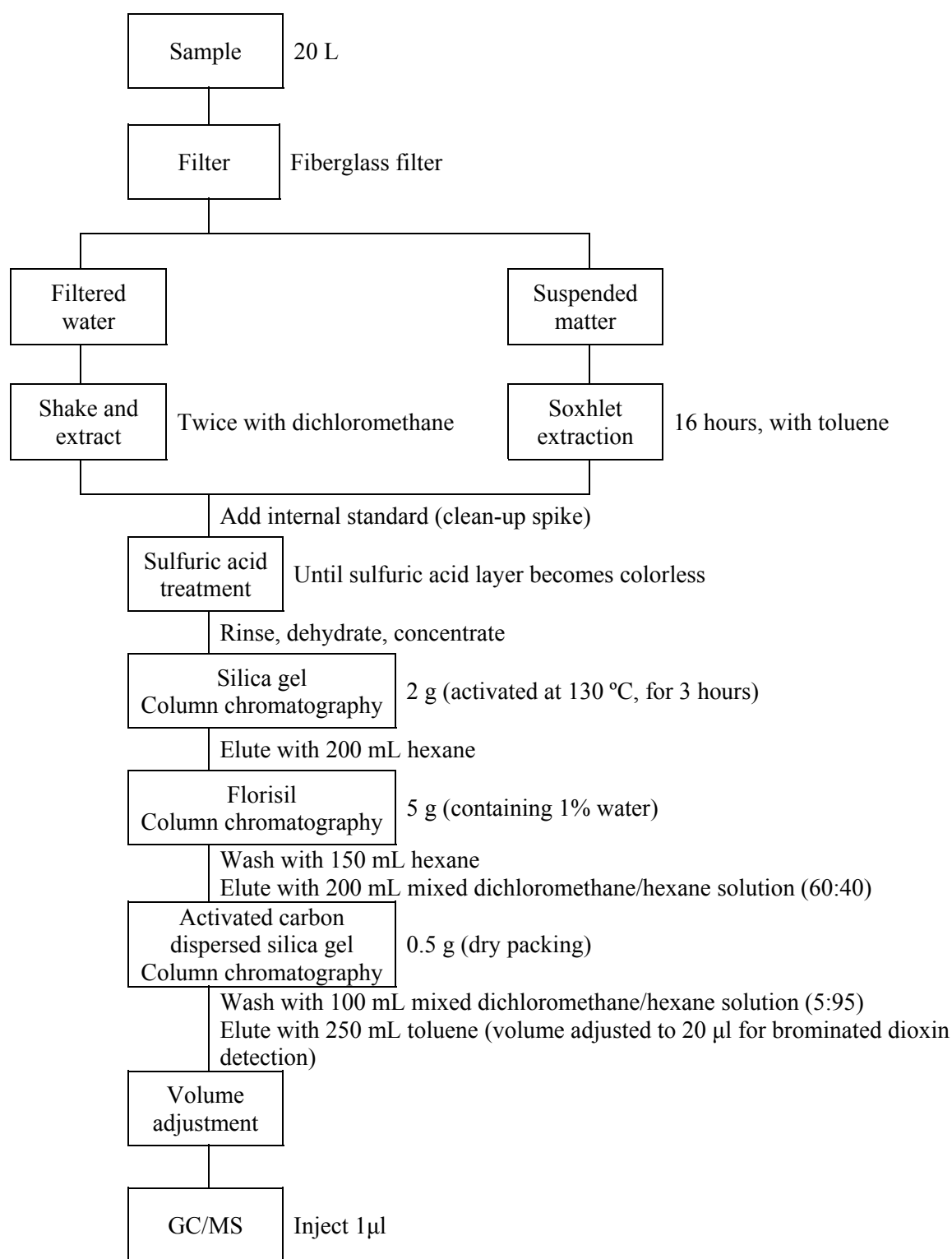
Figure 11. Flowchart of analytical method for determining brominated dioxins in groundwater and public water
