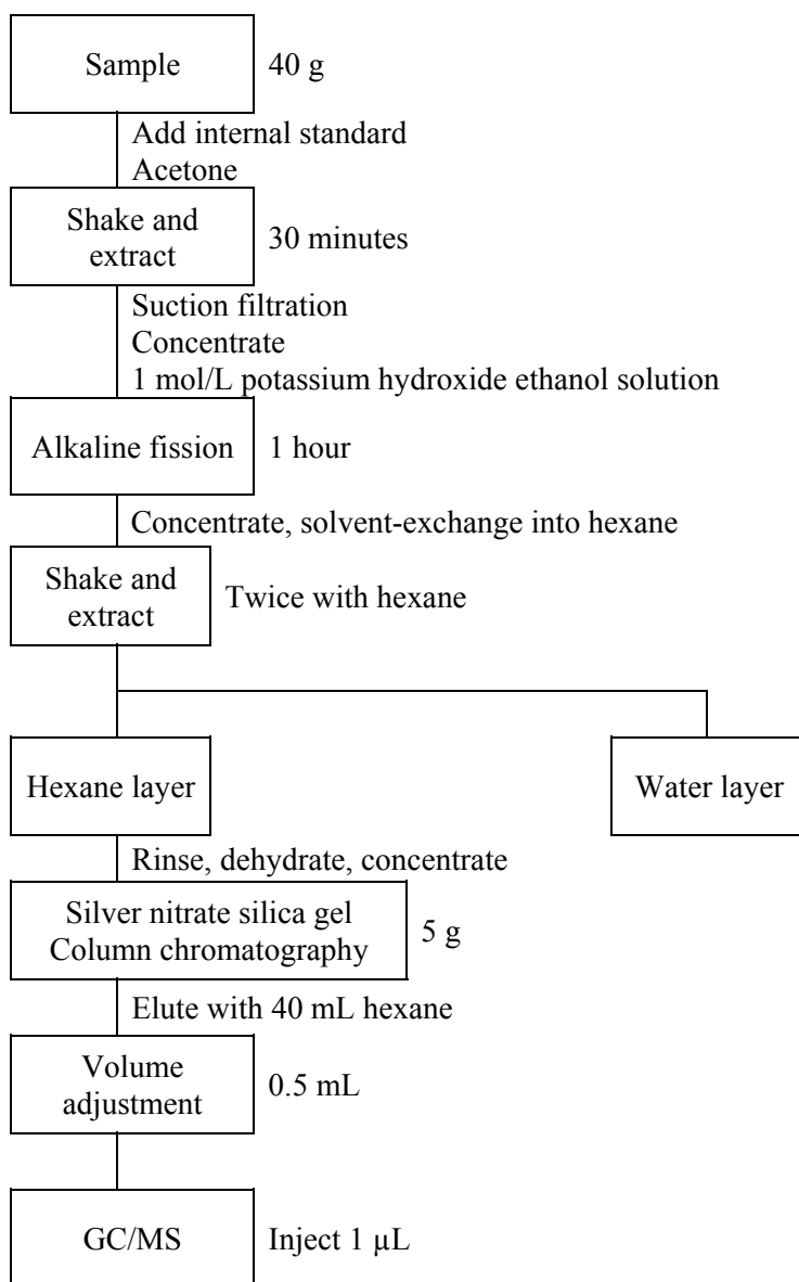
Figure 19. Flowchart of analytical method for determining polybrominated diphenyl ethers in food samples
