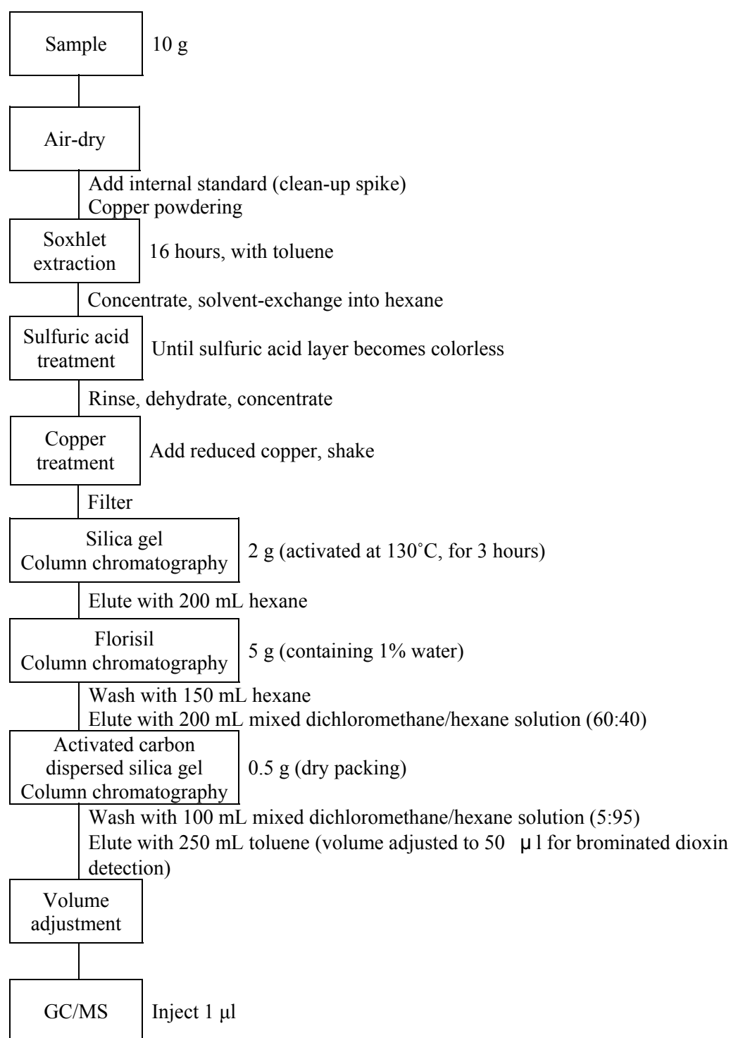
Figure 10. Flowchart of analytical method for determining brominated dioxins in soil and sediment
