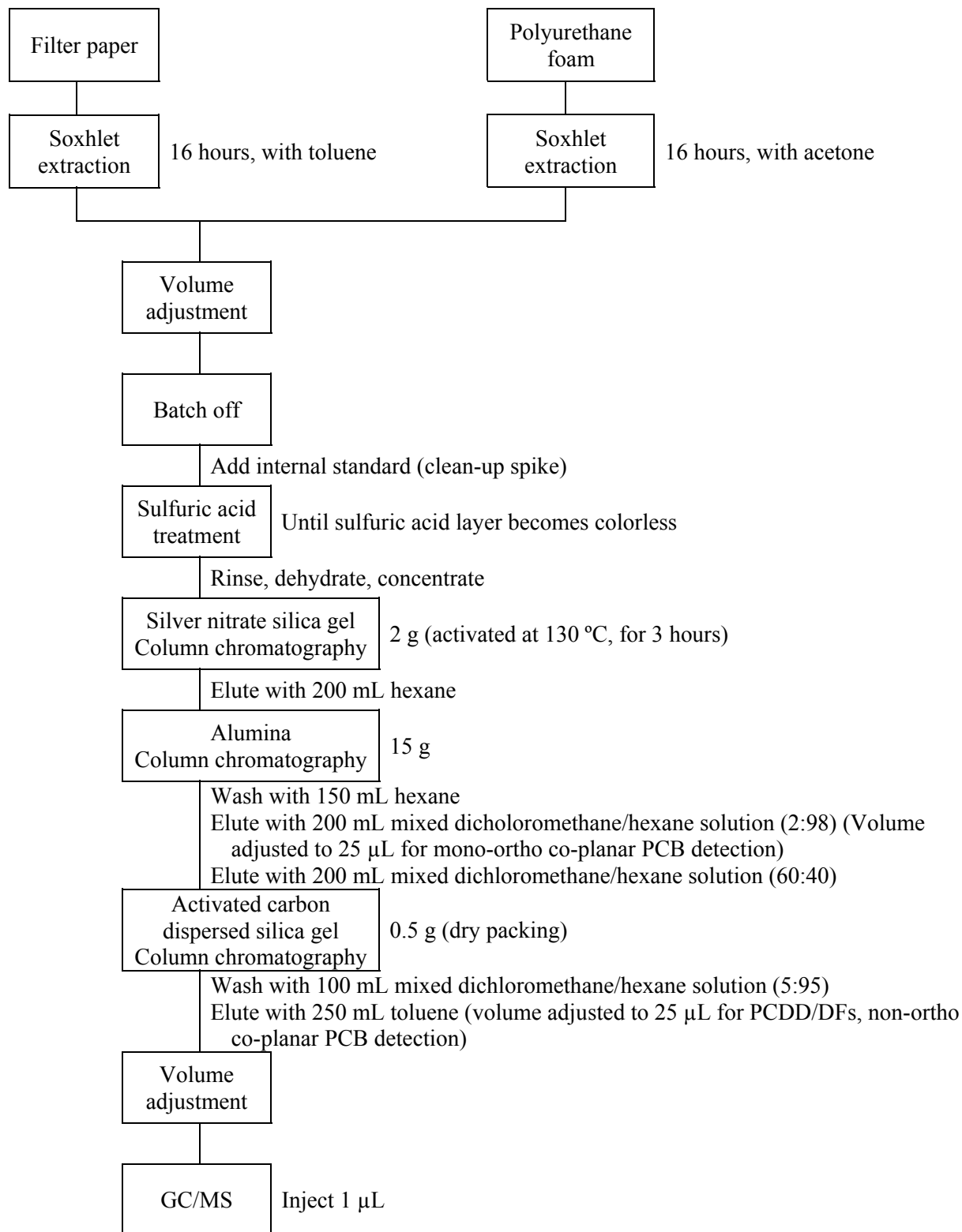
Figure 13. Flowchart of analytical method for determining (chlorinated) dioxins in ambient air and settled soot and dust
