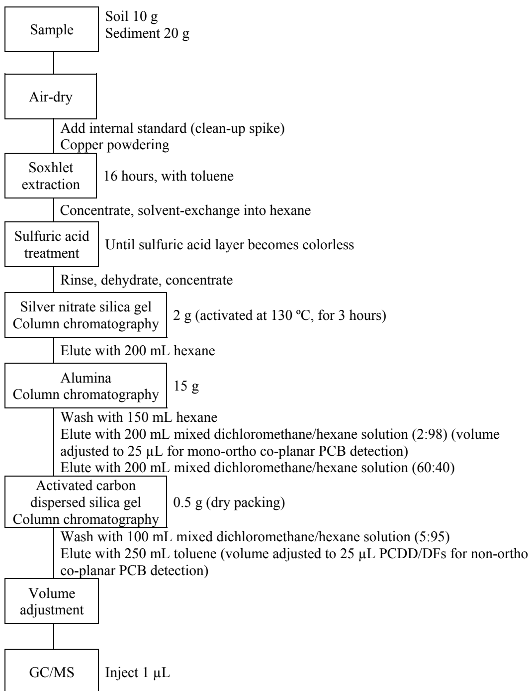
Figure 14. Flowchart of analytical method for determining (chlorinated) dioxins in soil and sediment
