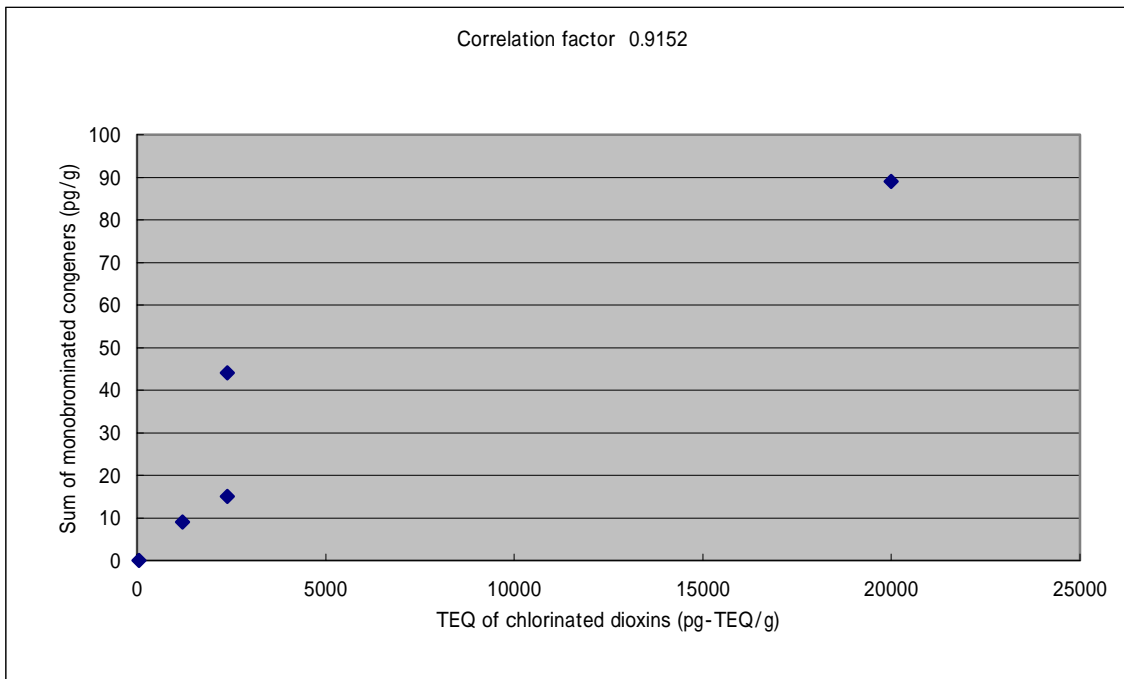
Figure 30. Correlation between sum of monobromopolychlorinated dioxin congeners and total (chlorinated) dioxins (sediment)
