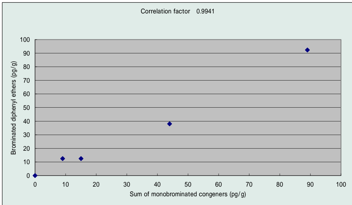
Figure 31. Correlation between sum of monobromopolychlorinated dioxin congeners and total polybrominated diphenyl ethers (sediment)
