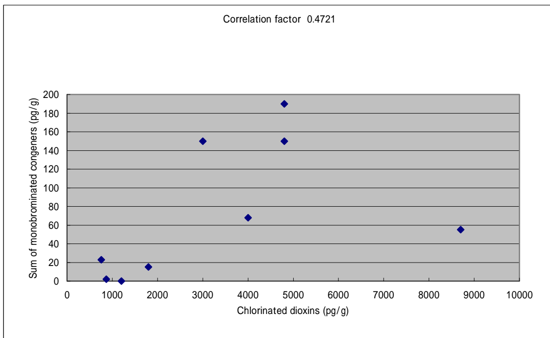
Figure 26. Correlation between sum of monobromopolychlorinated dioxin congeners and total (chlorinated) dioxins (soil)
