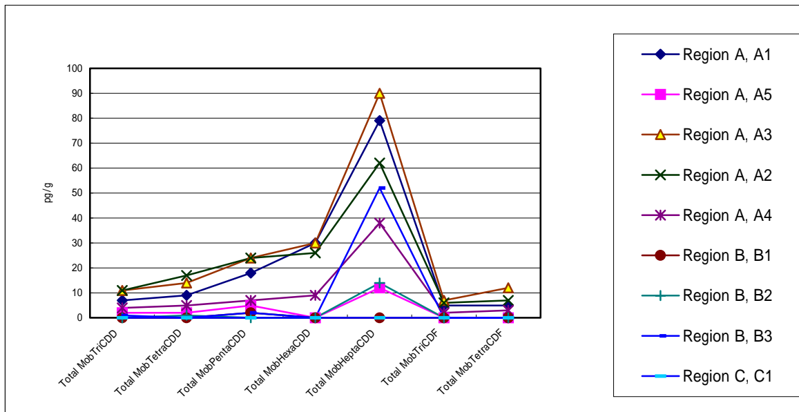
Figure 25. Distribution of monobromopolychlorinated dioxin congeners (soil)
