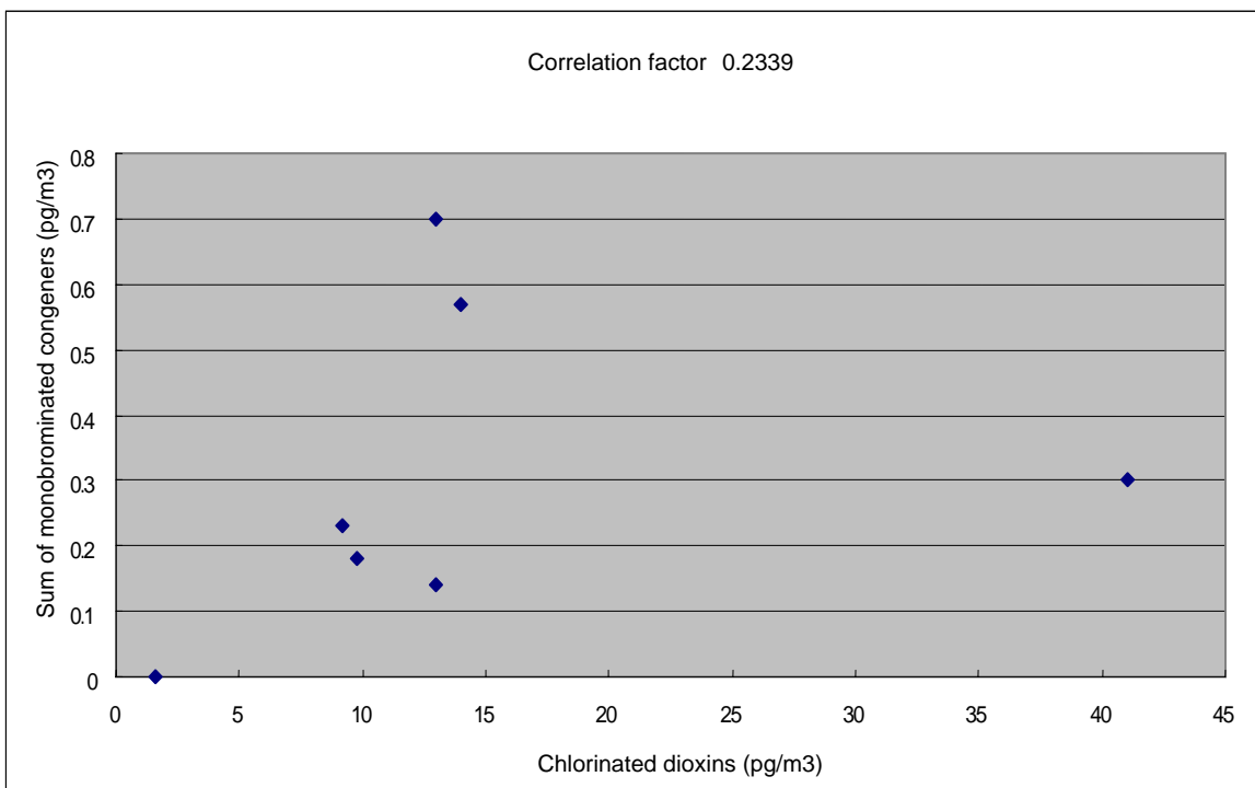
Figure 21. Correlation between sum of monobromopolychlorinated dioxin congeners and (chlorinated) dioxins (ambient air)
