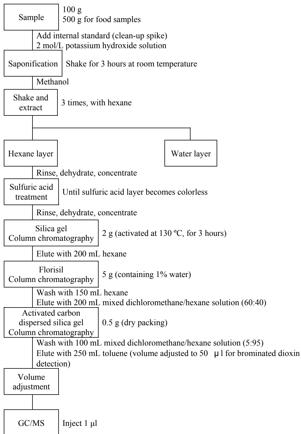
Figure 12. Flowchart of analytical method for determining brominated dioxins in aquatic life, terrestrial wildlife, and food samples
