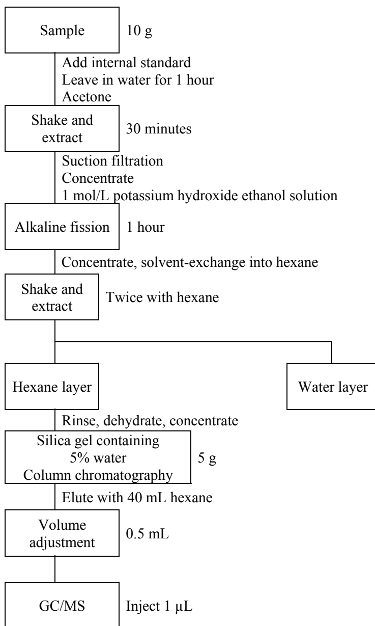
Figure 17. Flowchart of analytical method for determining polybrominated diphenyl ethers in soil
