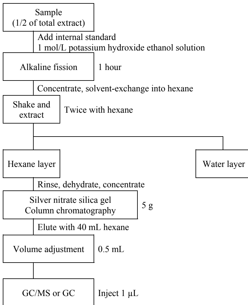
Figure 16. Flowchart of analytical method for determining polybrominated diphenyl ethers in ambient air and settled soot and dust
