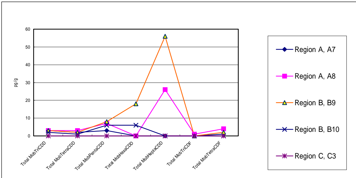
Figure 29. Distribution of monobromopolychlorinated dioxin congeners (sediment)
