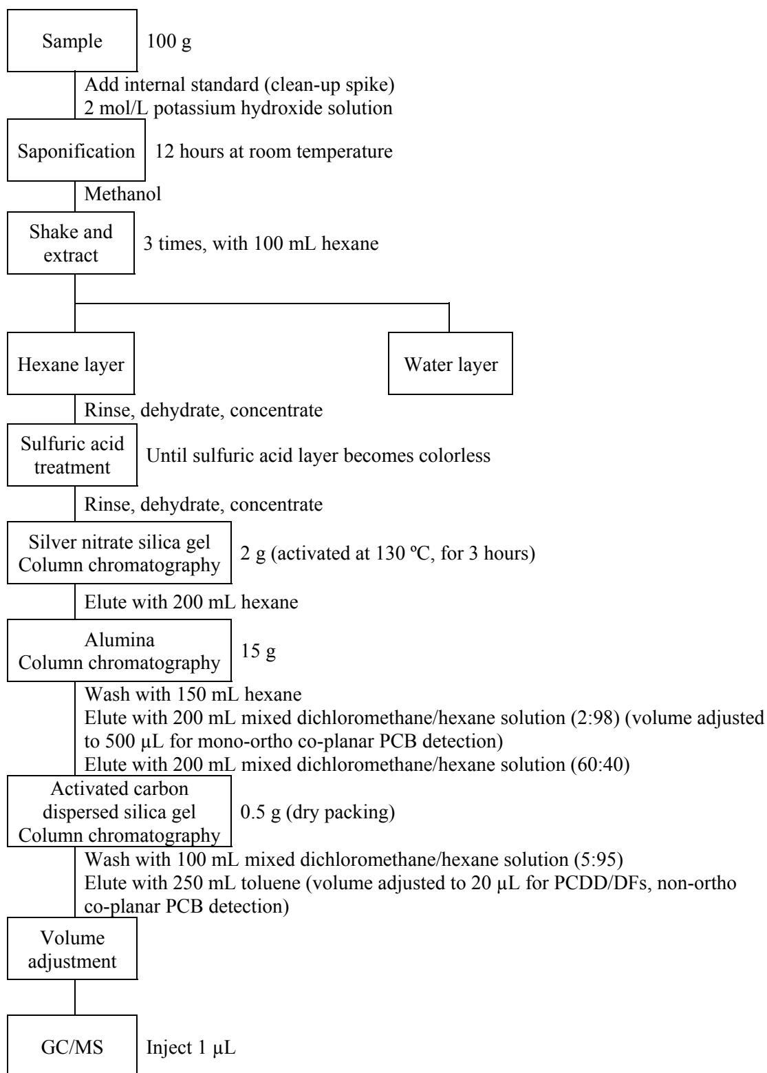
Figure 15. Flowchart of analytical method for determining (chlorinated) dioxins in food samples
