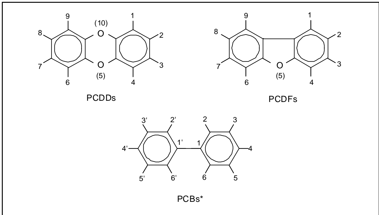
Fig. 1 Chemical Structure of Dioxins
