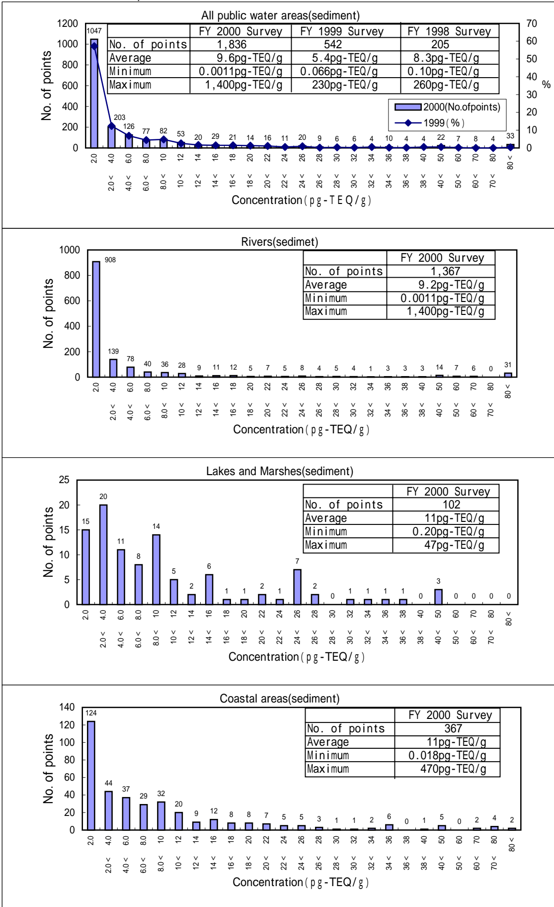
Figure 5: FY 2000 Results of Environmental Survey of Dioxins (Sediment in Public Water Areas)-Distribution of Concentrations
