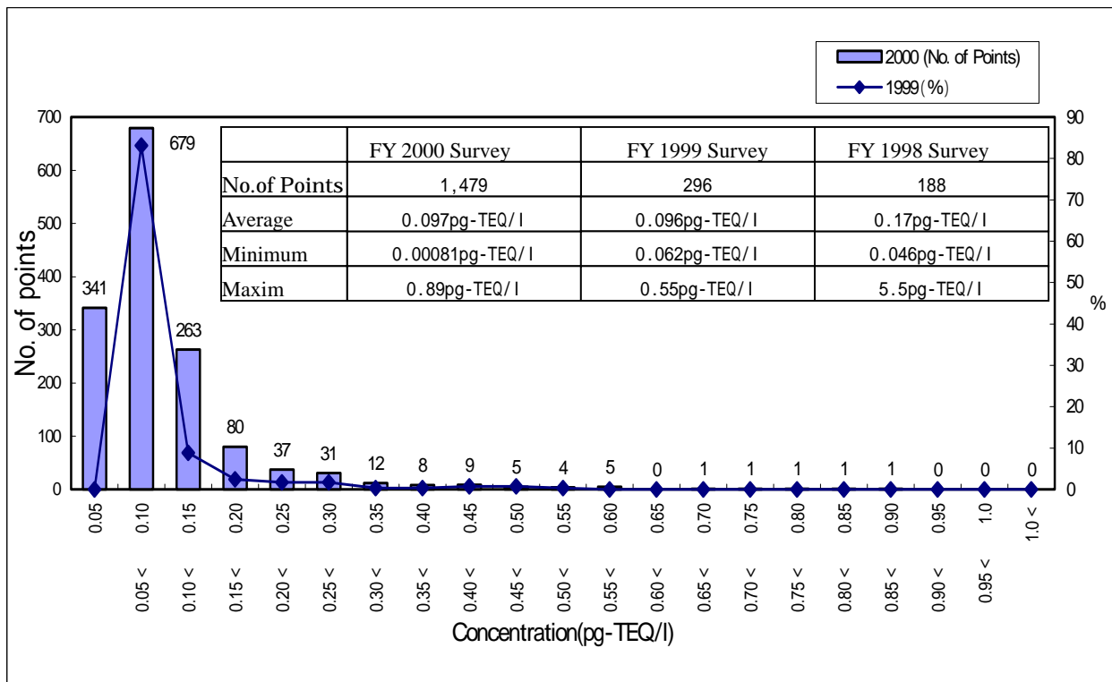
Figure 4: FY 2000 Results of Environmental Survey of Dioxins (Ground Water)—Distribution of Concentrations
