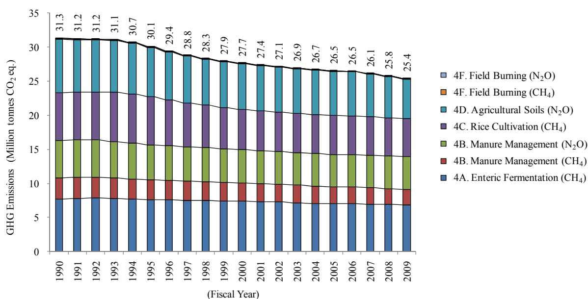
Figure 2-15 Trends in greenhouse gas emissions from the Agriculture sector
