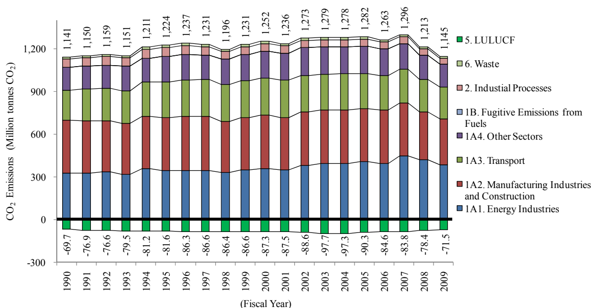
Figure 2-4 Trends in CO 2 emissions
