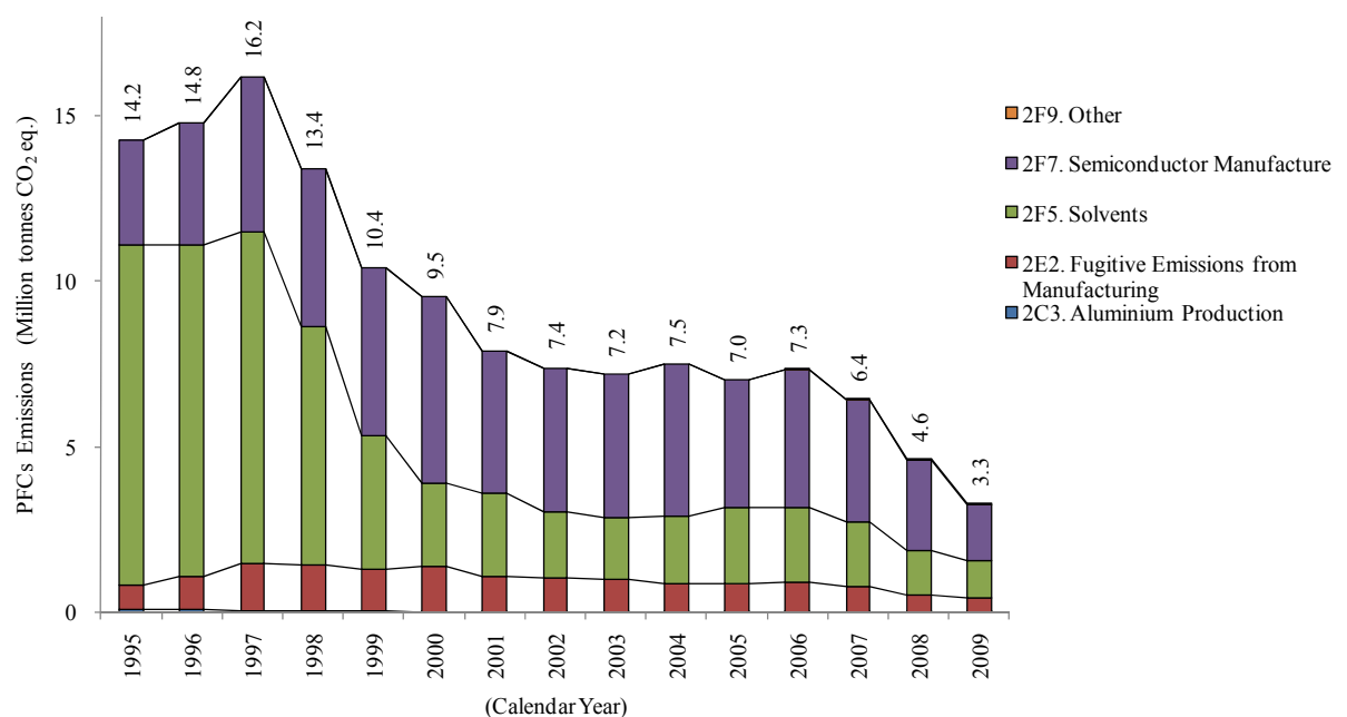
Figure 2-9 Trends in PFCs emissions
