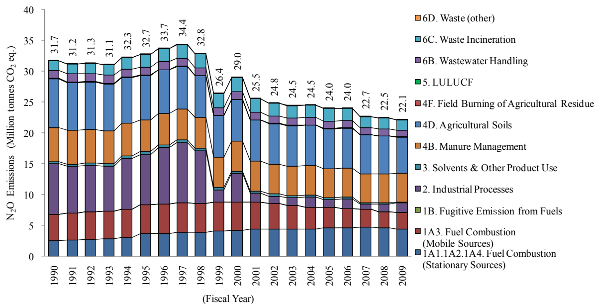
Figure 2-7 Trends in N 2 O emissions
