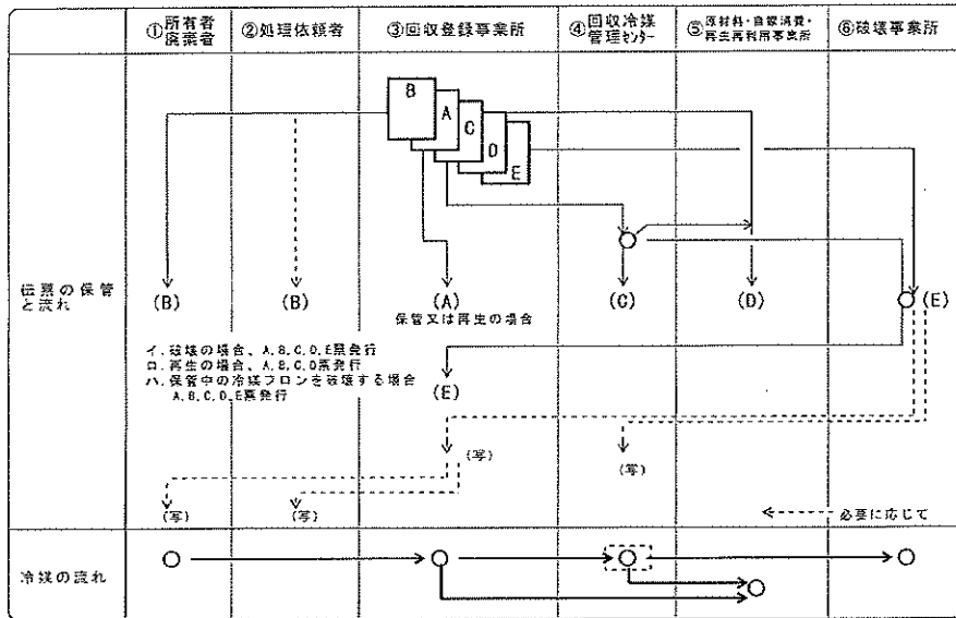
Fig. 8 Manifest sheet flow diagram
