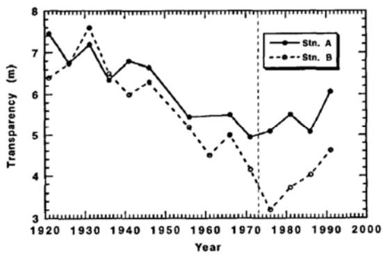
Figure 10 Chronological change in transparencies of five years average at Stations A. and B (see Figure 9) in the months between February and April from 1921 to 1991 (data source: see text). The vertical dashed line signifies the year when the law on the environmental conservation of the Seto Inland Sea was enacted.
