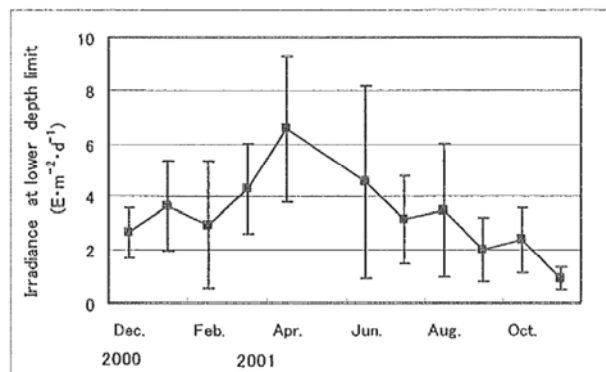
Fig. 2 Seasonal changes in irradiance at lower depth limit of eelgrass bed.
