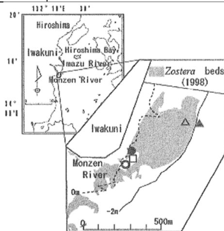
Fig. 1 Location map of the study area on the coast of Iwakuni in western Hiroshima Bay, the Seto Inland Sea, Japan. ●(vegetated), ○(unvegetated); measuring sites of sand movement, ▲; measuring sites of light intensity, △; sampling site of sediment deposition on leaves, □; transplantation site.
