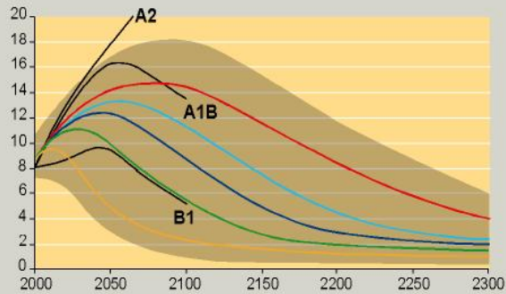
(a) CO 2 emissions (Gt C)
