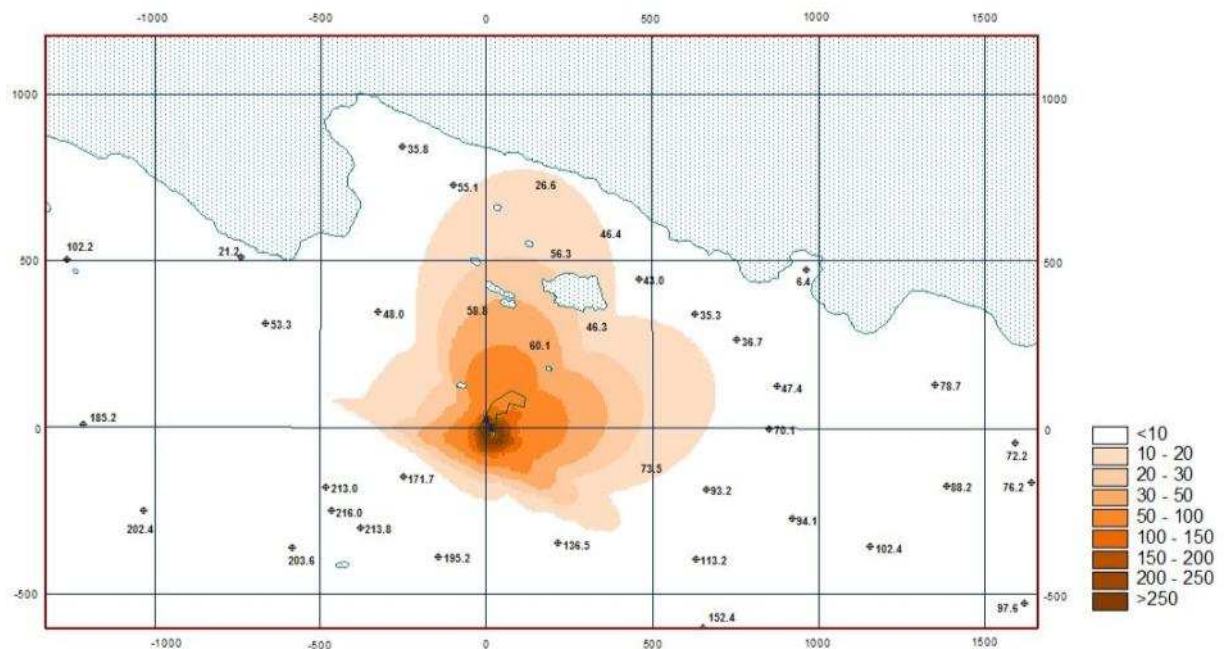
Figure 3 – Distribution of monthly average carbon oxide concentrations in atmospheric air from BAS stationary sources operation, \mu\text{g}/\text{m}^3 . Scenario 2
