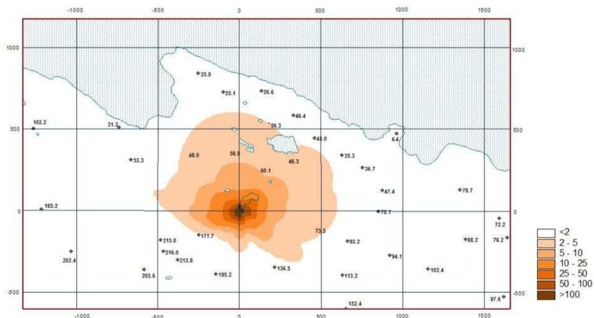
Figure 5 – Distribution of maximum 24-hour nitrogen dioxide concentrations in atmospheric air from BAS stationary sources operation, \mu\text{g}/\text{m}^3 . Scenario 2
