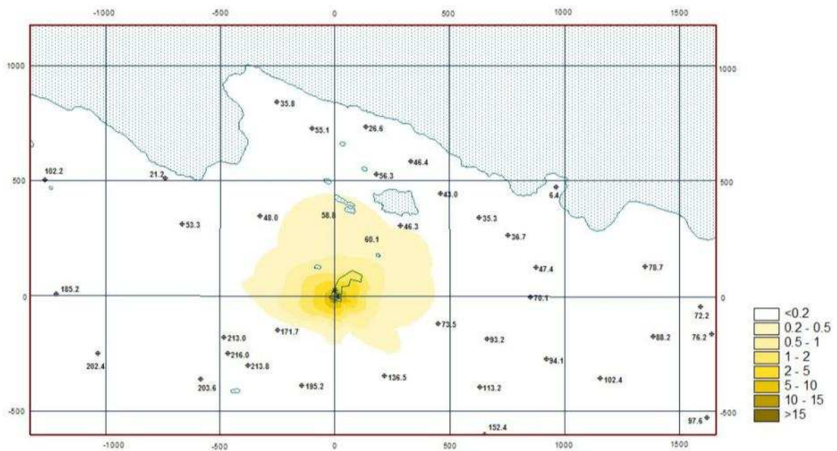
Figure 8 – Distribution of maximum 24-hour PM 10 concentrations in atmospheric air from BAS stationary sources operation, µg/m 3 . Scenario 2
