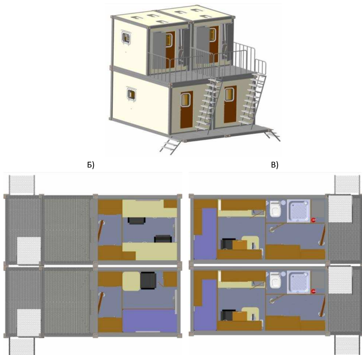
Figure 2.8 – General view (A) and layout (B) of the production & residential two-storey module
