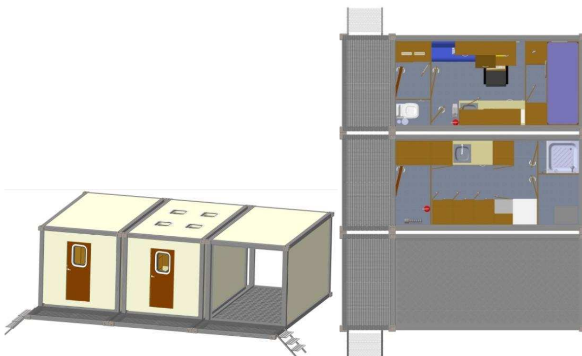
Figure 2.5 – General view (A) and layout (B) of the laboratory &amp; residential single-storey module
