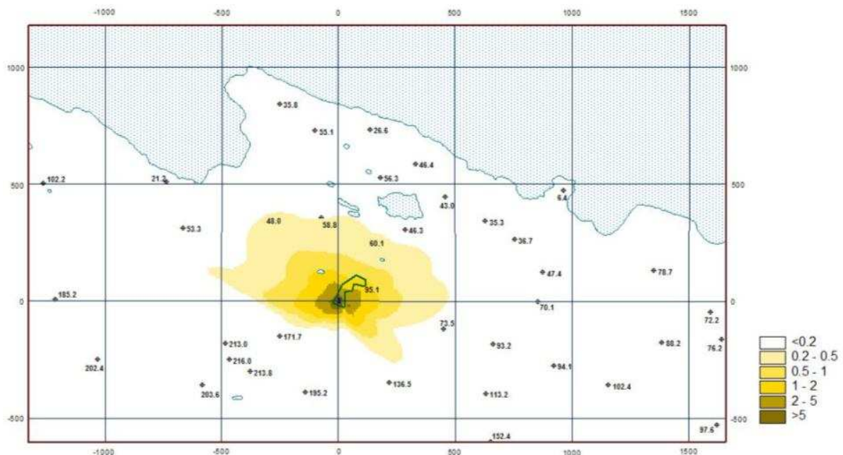
Figure 4.19 – Distribution of maximum 24-hour PM 10 concentrations in atmospheric air from BAS stationary sources operation, µg/m 3 . Scenario 1
