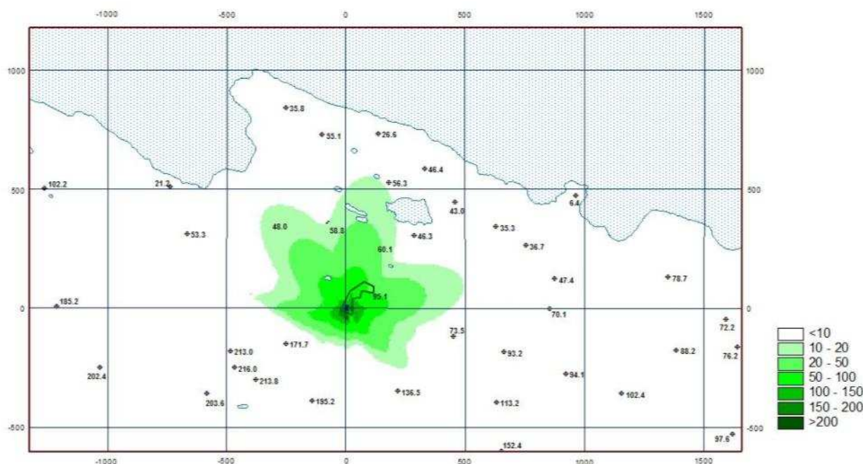
Figure 4.12 - Distribution of maximum 1-hour CO concentrations in atmospheric air from BAS stationary sources operation, \mu\text{g}/\text{m}^3 . Scenario 1
