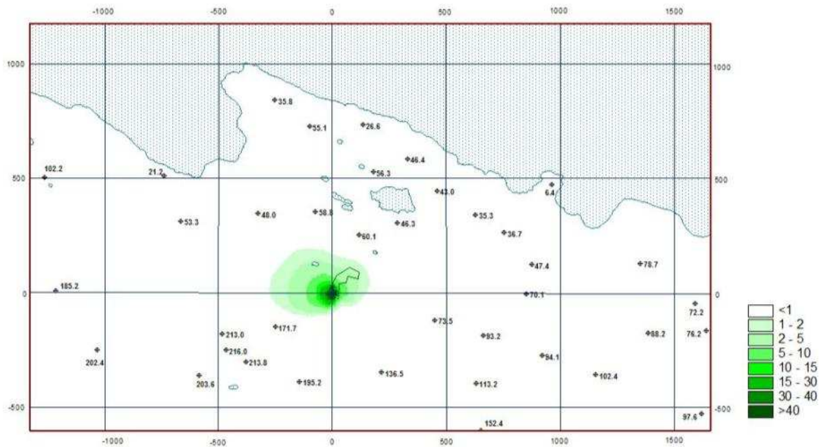
Figure 3 – Distribution of monthly average carbon oxide concentrations in atmospheric air from BAS stationary sources operation, \mu\text{g}/\text{m}^3 . Scenario 2
