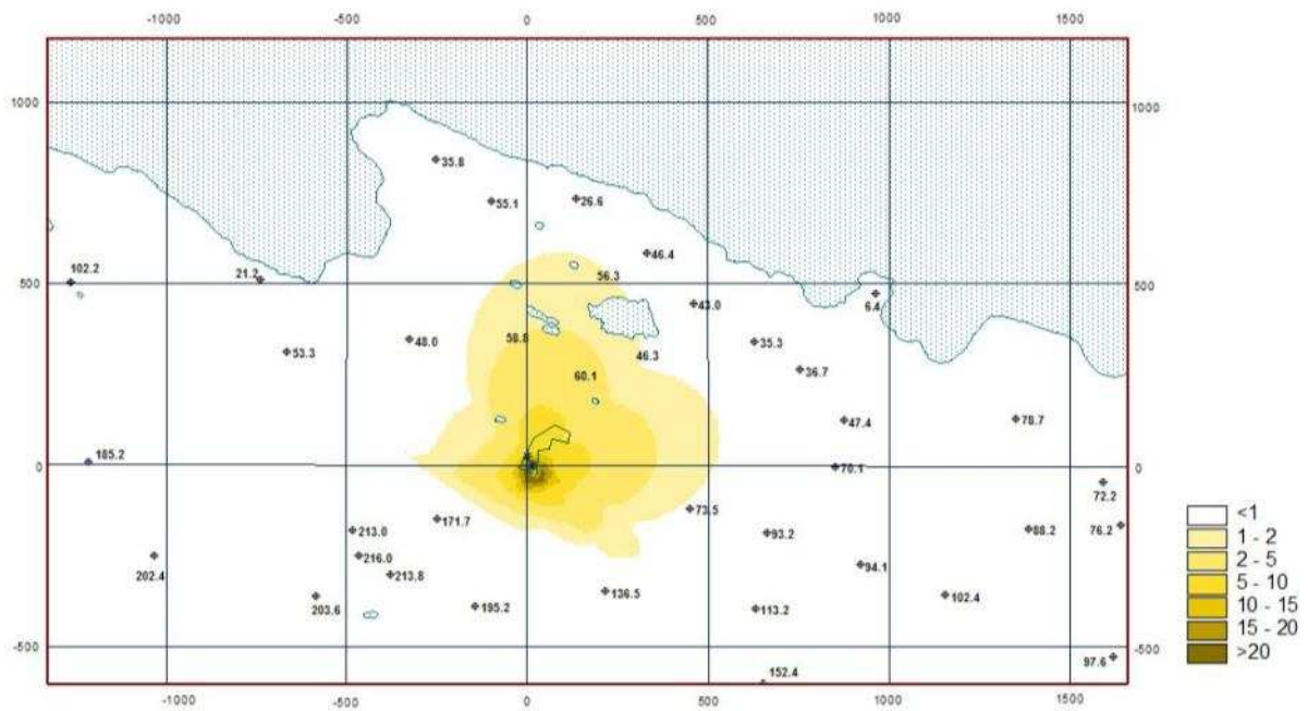
Figure 7 – Distribution of maximum 1-hour PM 10 concentrations in atmospheric air from BAS stationary sources operation, µg/m 3 . Scenario 2
