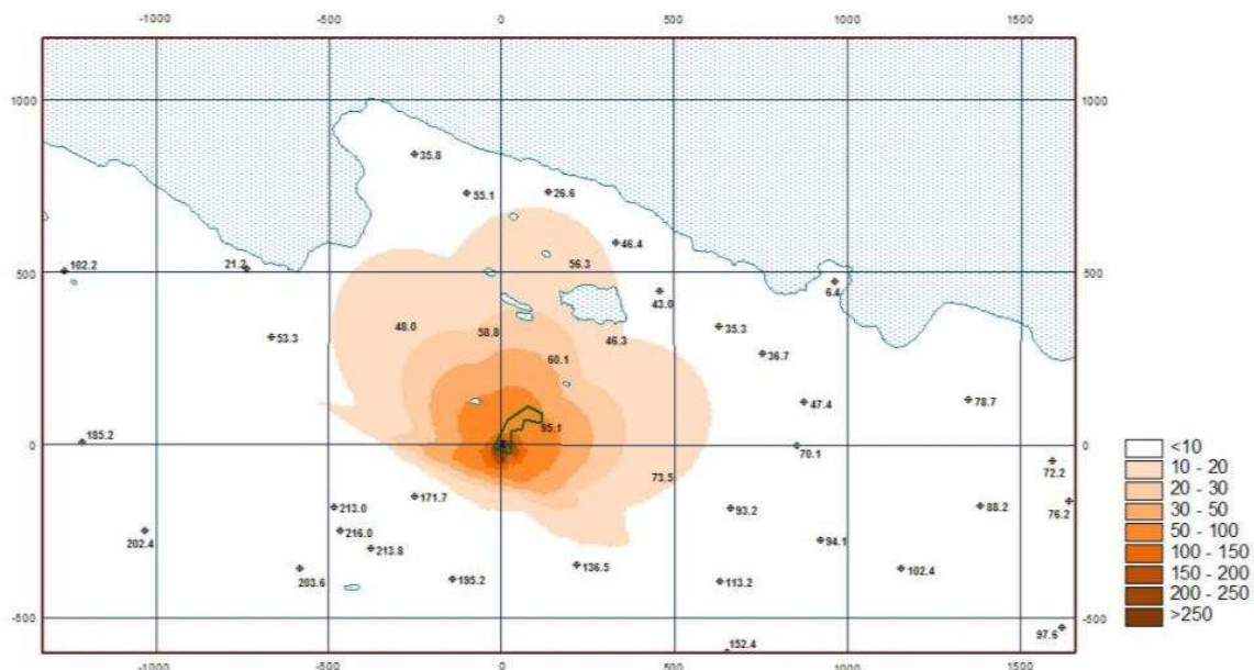
Figure 4.15 – Distribution of maximum hourly \text{NO}_2 concentrations in atmospheric air from BAS stationary sources operation, \mu\text{g}/\text{m}^3 . Scenario 1
