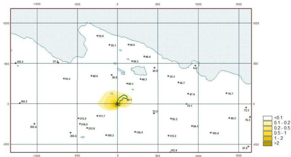
Figure 4.20 – Distribution of monthly average PM 10 concentrations in atmospheric air from BAS stationary sources operation, averaged for summer seasons (December-March), \mu\text{g}/\text{m}^3 , Scenario 1
