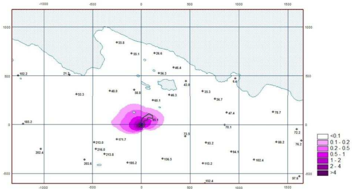
Figure 4.23 – Distribution of monthly average \text{SO}_2 concentrations in atmospheric air from BAS stationary sources operation, averaged for summer seasons (December-March), \mu\text{g}/\text{m}^3 , Scenario 1
