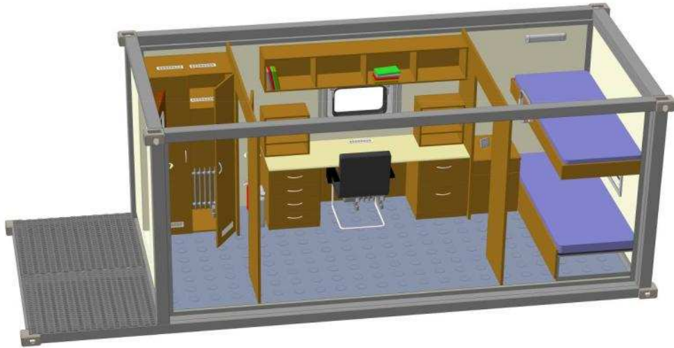
Figure 3 - Left section of the module. Right-side view From the entrance: a lobby, wardrobe with heating elements, lab workplace, compartment for recreation.
