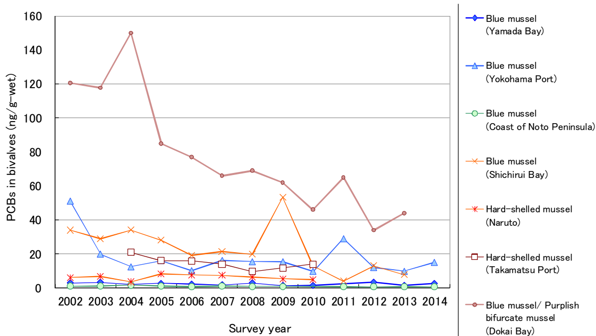
Figure 3: Temporal trends of PCBs concentrations in bivalves
