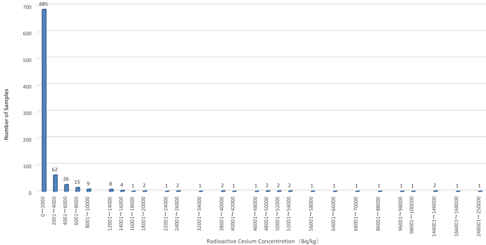
Lakes(Sediment):Number of Samples by redioactive cesium concentretion(2000Bg/kg)(FY2021)
