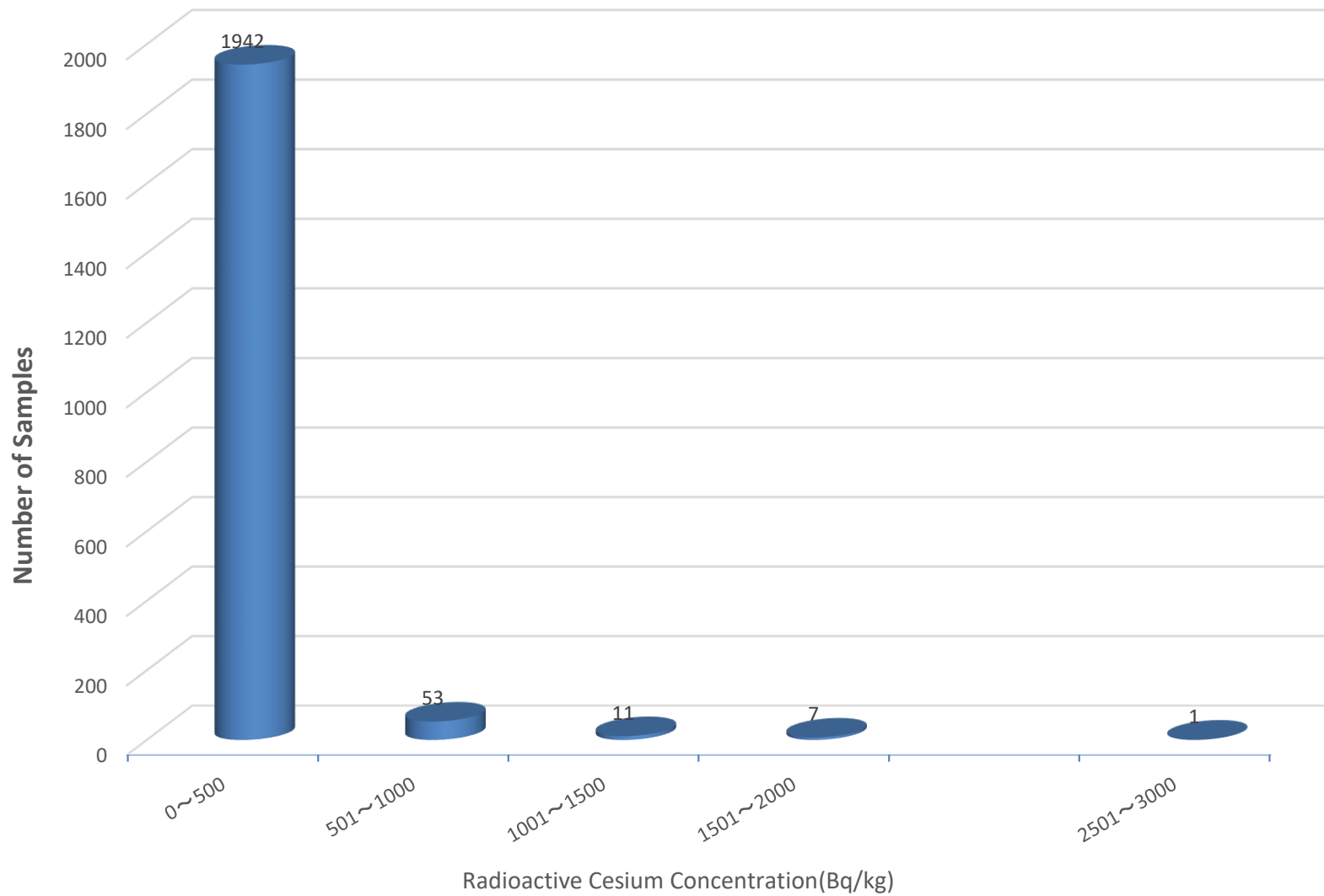
Rivers(Sediment):Number of Samples by radioactive cesium concentration (500Bq/kg)(FY2021)
