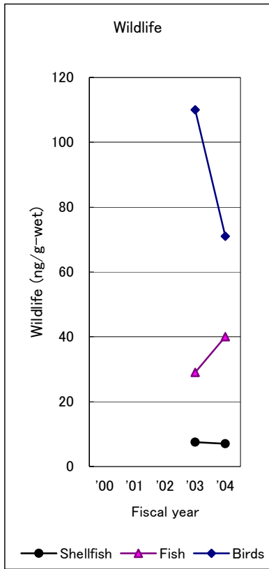
Figure 4-23-A Annual Change of Toxaphene (Parlar 26) in Wildlife (fish, shellfish, birds) (geometric mean)
