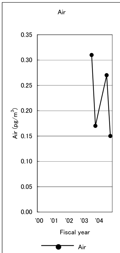
Figure 4-23-B Annual Change of Toxaphene (Parlar 26) in Air (geometric mean)
