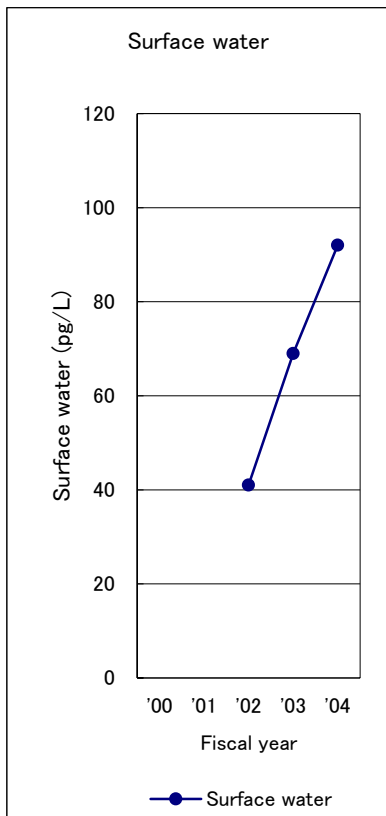
Figure 4-17-A Annual Change of cis -Chlordane in Surface Water (geometric mean)
