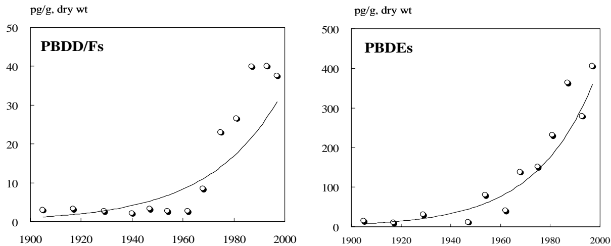
Figure 1. Temporal trends of concentrations of PBDD/Fs and PBDEs in the sediment cores from Tokyo Bay
